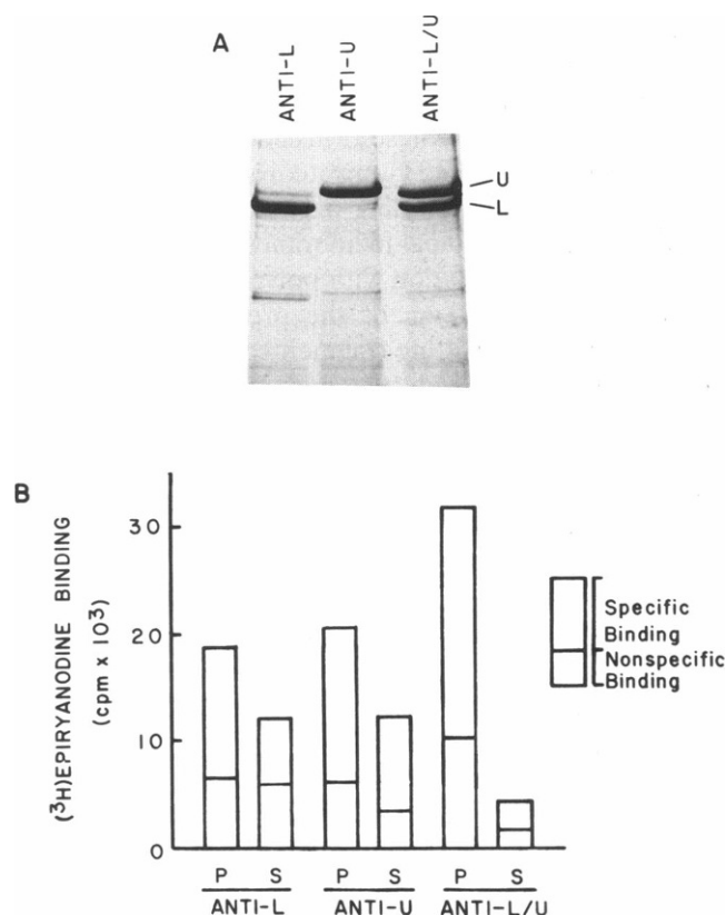
FIGURE 4 Bullfrog hindlimb muscle sarcoplasmic reticulum contains two homooligomeric, high molecular mass proteins that bind [ ^3\text{H} ]epiryanodine. The large molecular mass proteins were solubilized from microsomal membranes with CHAPS and precipitated using monoclonal antibodies that recognize either only one (Mab 26G = anti-L; Mab 29F = anti-U) or both of the high molecular mass polypeptides (Mab 34C = antiL/U). (A) Immunoprecipitated proteins were resolved in continuous 4–20% polyacrylamide gradient SDS gels and visualized after staining with Coomassie brilliant blue. U and L refer to the higher and lower molecular mass polypeptides, respectively. The molecular mass standards were the same as those described for Fig. 1. (B) The solubilized proteins were incubated with [ ^3\text{H} ]epiryanodine before immunoprecipitation. The level of binding associated with the precipitates (P) and remaining in the supernatants (S) after precipitation with either polypeptide specific, or an antibody that recognizes both polypeptides were measured.
