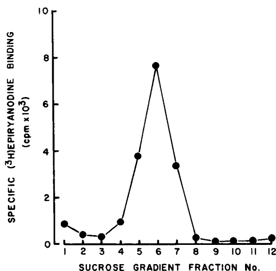
FIGURE 3 Specific [ ^3\text{H} ]epiryanodine binding copurifies with the high molecular mass proteins solubilized from bullfrog hindlimb muscle sarcoplasmic reticulum membranes. Equal volumes of the sucrose gradient fractions shown in Fig. 2A, were tested for the ability to bind [ ^3\text{H} ]epiryanodine as described in Experimental Procedures.
