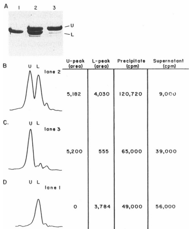
FIGURE 8 The two foot protein isoforms in chicken pectoral muscle bind approximately equivalent levels of [ ^3\text{H} ]epiryanodine. An experiment identical to that described in Fig. 7 was conducted using chicken pectoral muscle microsomal membranes. In this study, Mab 110F = anti-U; Mab 110E = anti-L; and Mab 34C = anti-L/U.
