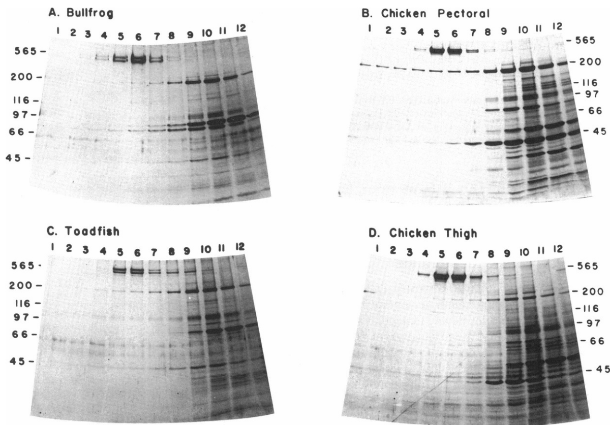
FIGURE 2 The sarcoplasmic reticulum in nonmammalian vertebrate muscle contains large proteins with comparable native and polypeptide subunit sizes. Proteins in microsomal membranes obtained from bullfrog hindlimb ( A ), chicken pectoral ( B ), toadfish back ( C ), and chicken thigh ( D ) were solubilized with CHAPS and sedimented through continuous 10–30% sucrose gradients as described in Experimental Procedures. The gradients were fractionated and the protein profiles of each fraction (numbered from the bottom of the gradient) determined using SDS-PAGE and staining with Coomassie brilliant blue. Comparable amounts of protein were loaded onto each gradient. The molecular mass standards used are those described for Fig. 1.
