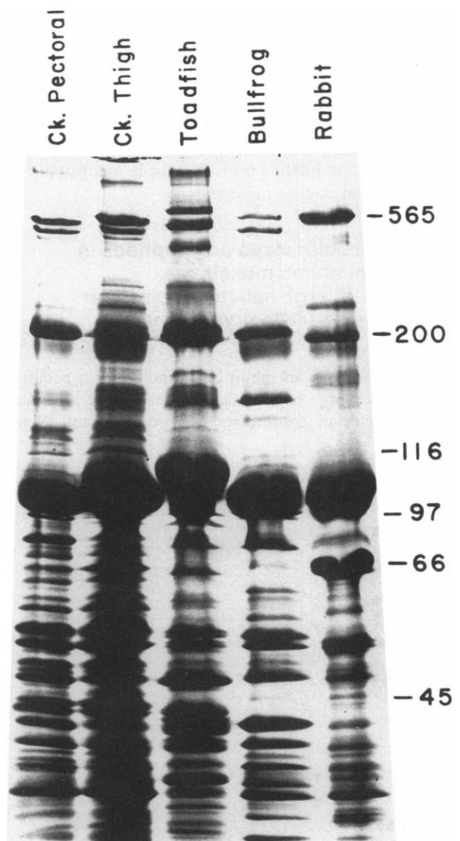
FIGURE 1 Multiple high molecular mass polypeptides are present in sarcoplasmic reticulum from nonmammalian vertebrate skeletal muscles. The proteins in microsomal membranes isolated from chicken pectoral (80 µg) and thigh (70 µg), toadfish back (80 µg), bullfrog hindlimb (50 µg), and rabbit back (37.5 µg) muscles were separated in a continuous 4–20% polyacrylamide gradient SDS gel and visualized by staining with Coomassie brilliant blue. The rabbit skeletal muscle foot protein (565 kD), myosin heavy chain (200 kD), beta-galactosidase (116 kD), phosphorylase b (98 kD), BSA (66 kD) and ovalbumin (45kD) were used as molecular mass standards.
