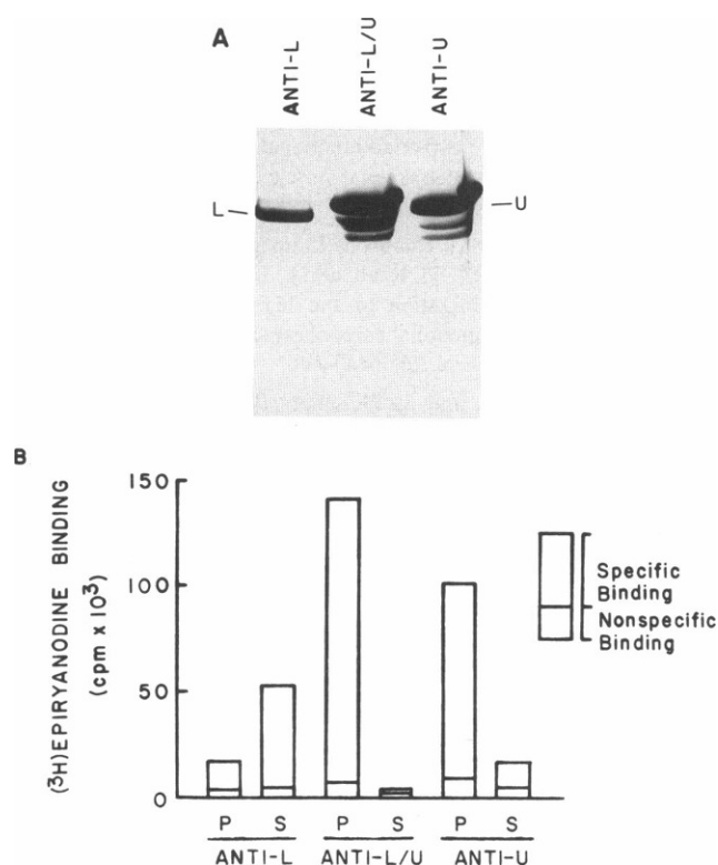
FIGURE 9 Chicken thigh muscle also contains two homooligomeric ryanodine binding proteins. (A) Microsomal membrane proteins were solubilized with CHAPS and precipitated with monoclonal antibodies specific for the larger polypeptide subunit (Mab 110F = anti-U), the smaller subunit (Mab 110E = anti-L), or both polypeptides (Mab 34C = anti-L/U). The precipitated polypeptides were separated in a continuous 4–20% polyacrylamide gradient SDS gel and visualized after staining with Coomassie brilliant blue. (B) In a parallel experiment, the solubilized proteins were incubated with [ ^3 H]epiryanodine before immunoprecipitation and the levels of bound ligand in the precipitates (P) and remaining in the supernatants (S) were determined in each case.
