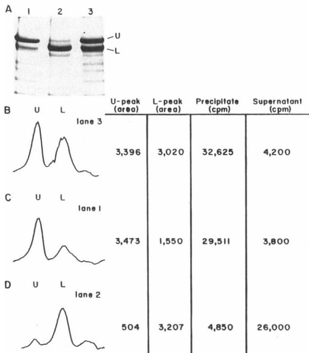
FIGURE 7 Toadfish skeletal muscle sarcoplasmic reticulum contains two homooligomeric proteins which both bind [ ^3\text{H} ]epiryanodine. (A) Toadfish muscle microsomal membrane protein was solubilized with CHAPS and immunoprecipitated with monoclonal antibodies specific for either the larger (Mab 34C = anti-U, lane 1), or smaller (L, Mab 59E = anti-L, lane 2) polypeptide subunit, or with an antibody that recognizes both polypeptides (Mab 76F = anti-L/U, lane 3). The precipitated proteins were resolved in a continuous 4–20% polyacrylamide gradient gel and visualized after staining with Coomassie brilliant blue. (B–D) The high molecular mass proteins present in each lane in A were quantitated by densitometric scanning and the areas under each peak given in relative units. In a parallel experiment, the solubilized proteins were incubated with [ ^3\text{H} ]epiryanodine before immunoprecipitation. The levels of specifically bound ligand in both the precipitates and remaining in the supernatant after precipitation were determined.
