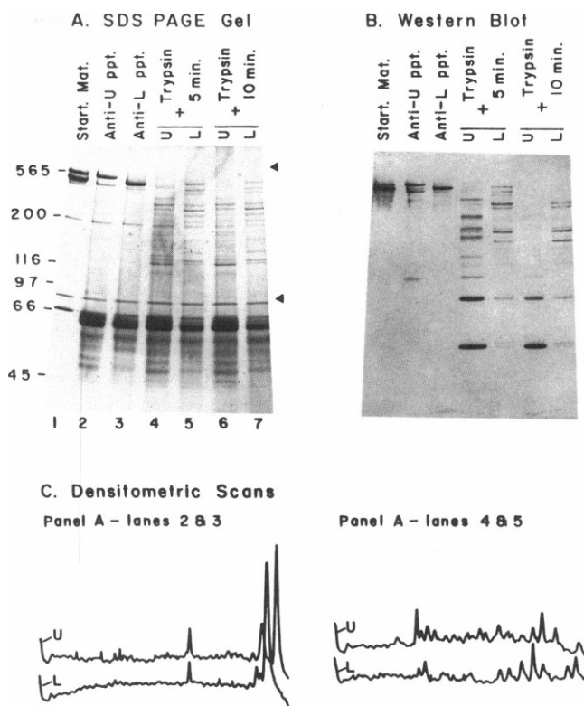
FIGURE 5 The two ryanodine-binding proteins in bullfrog skeletal muscle sarcoplasmic reticulum are unique and not related in a simple way by proteolysis. ( A ) Microsomal membrane protein was solubilized with CHAPS and sedimented through a continuous 10–30% sucrose gradient. Monoclonal antibodies specific for each polypeptide (Mab 26G = anti-L; Mab 29F = anti-U) were used to selectively precipitate each protein from an appropriate sucrose gradient fraction (lanes 1–3). The ratios of antibody and solubilized protein were adjusted to result in the precipitation of approximately equivalent quantities of each protein. The precipitates were incubated with trypsin (0.5 µg/ml) for either 5 or 10 min, at which time proteolysis was stopped by the addition of DFP (2 mM) and 4× SDS gel load buffer. The proteolytic fragments generated in each reaction were resolved in continuous 4–20% polyacrylamide gradient SDS gels (lanes 4–7) and visualized by staining with Coomassie brilliant blue. The molecular mass standards used are the same as those described for Fig. 1. ( B ) The proteins present in an SDS gel identical to that shown in A were electrophoretically transferred onto nitrocellulose and probed with a monoclonal antibody (Mab 34C) that recognizes both the larger ( U ) and smaller ( L ) polypeptide subunits. ( C ) The proteins present before ( left scan ) and after ( right scan ) proteolysis of precipitates containing either the larger ( U ) and smaller ( L ) polypeptide subunits were also visualized as densitometric scans of the region of the gel shown in A indicated by the arrowheads on the right side of the figure. The scan proceeded from left to right, starting at the lower arrowhead.
